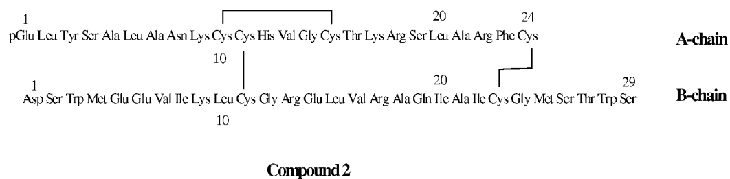
Figure 2. Structure (sequence) of synthetic human Relaxin 2 (shRLX2)
