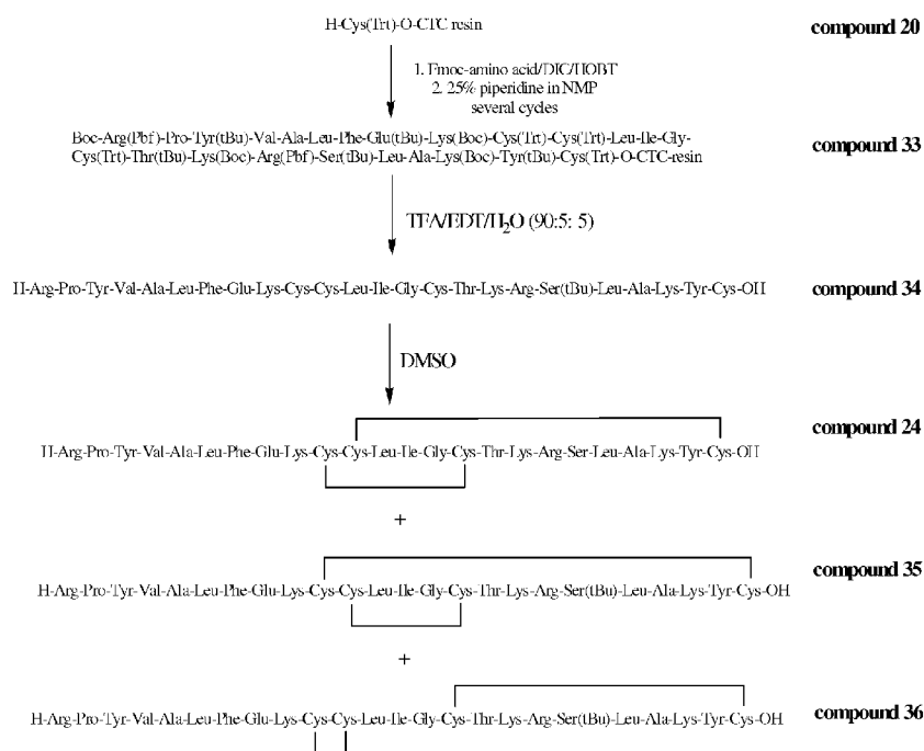
Figure 13. Synthesis of a mixture of bicyclic synthetic human relaxin I chains A [compounds 24, 35-36; bicyclic RLX1A] by the DMSO oxidation of the linear chain
