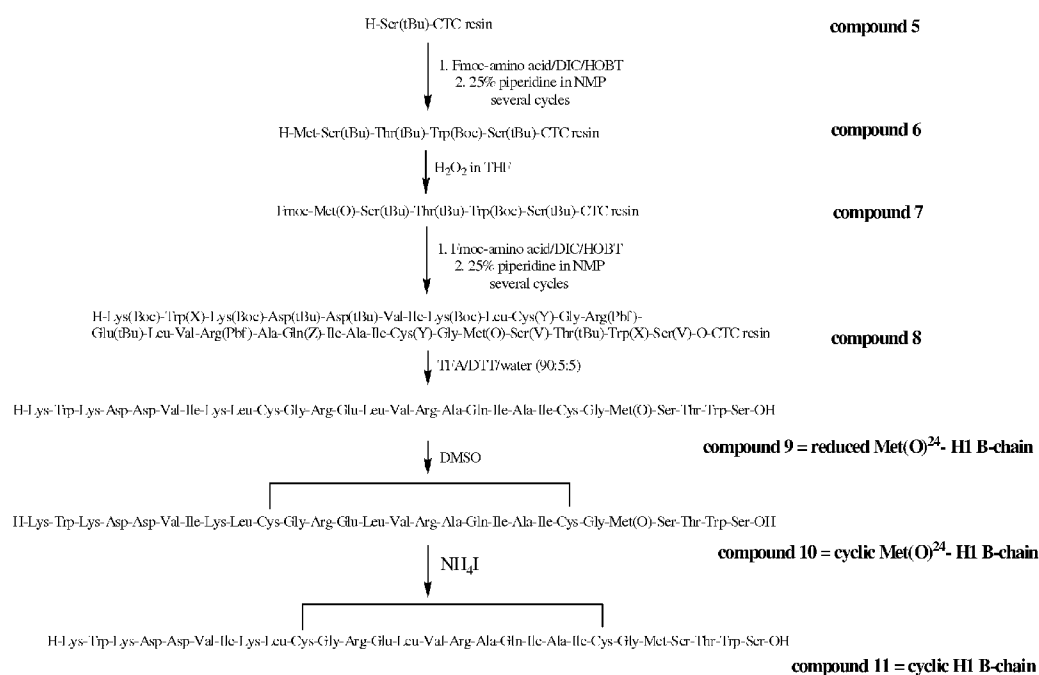
Figure 5. DMSO oxidation; Synthesis of reduced (linear) Met(O) 24 -human Relaxin 1 B-chain [ compound 9 , Met(O) 24 -shRI.X1B], of oxidized (cyclic) Met(O) 24 -human Relaxin 1 B-chain [ compound 10 , Met(O) 24 -shRI.X1B] and of oxidized (cyclic) human Relaxin 1 B-chain [ compound 11 , shRI.X1B]
