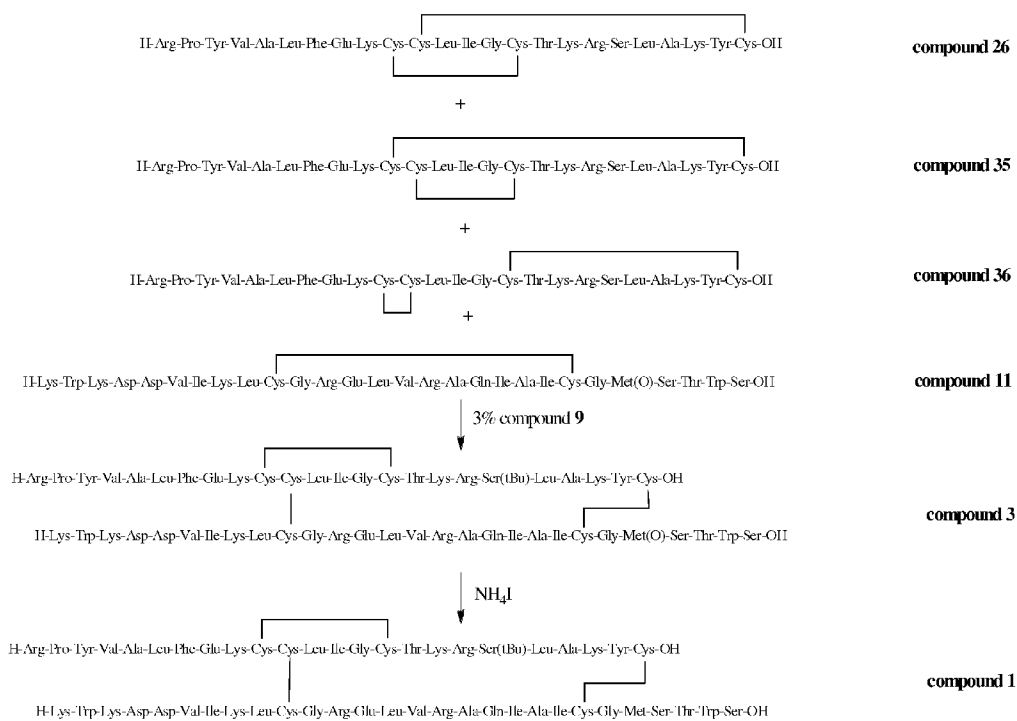
Figure 17. Synthesis of Met(O) 24 -Relaxin 1 [Met(O) 24 -RLX1] and of Relaxin 1 [RLX1] by chain combination of bicyclic RLX1A and cyclic RLX1B-chains
