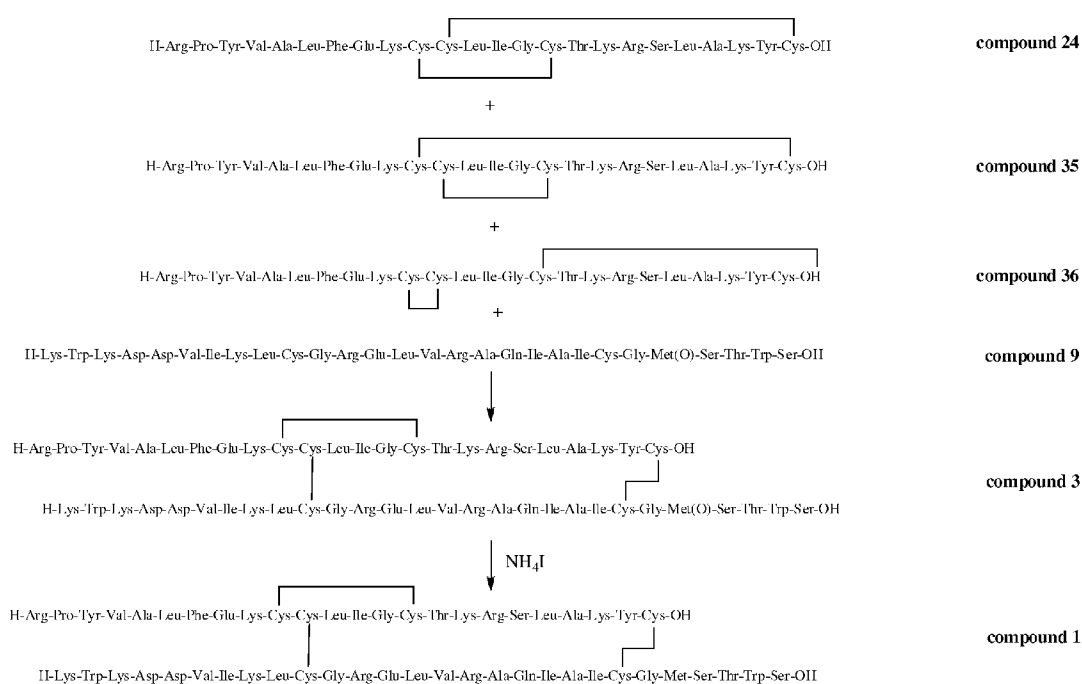
Figure 16. Synthesis of Met(O) 24 -Relaxin 1 [Met(O) 24 -RLX1; compound 3 ] and of Relaxin 1 [RLX1; compound 1 ] by chain combination of bicyclic R1X1A and reduced R1X1B-chains
