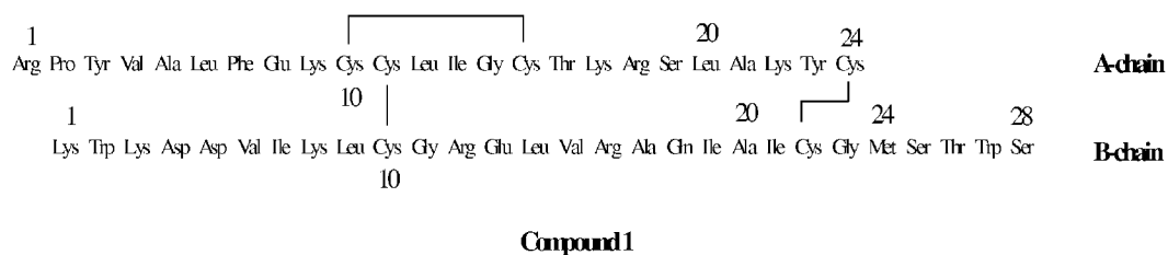
Figure 1. Structure (sequence) of synthetic human Relaxin 1 (shRLX1)
