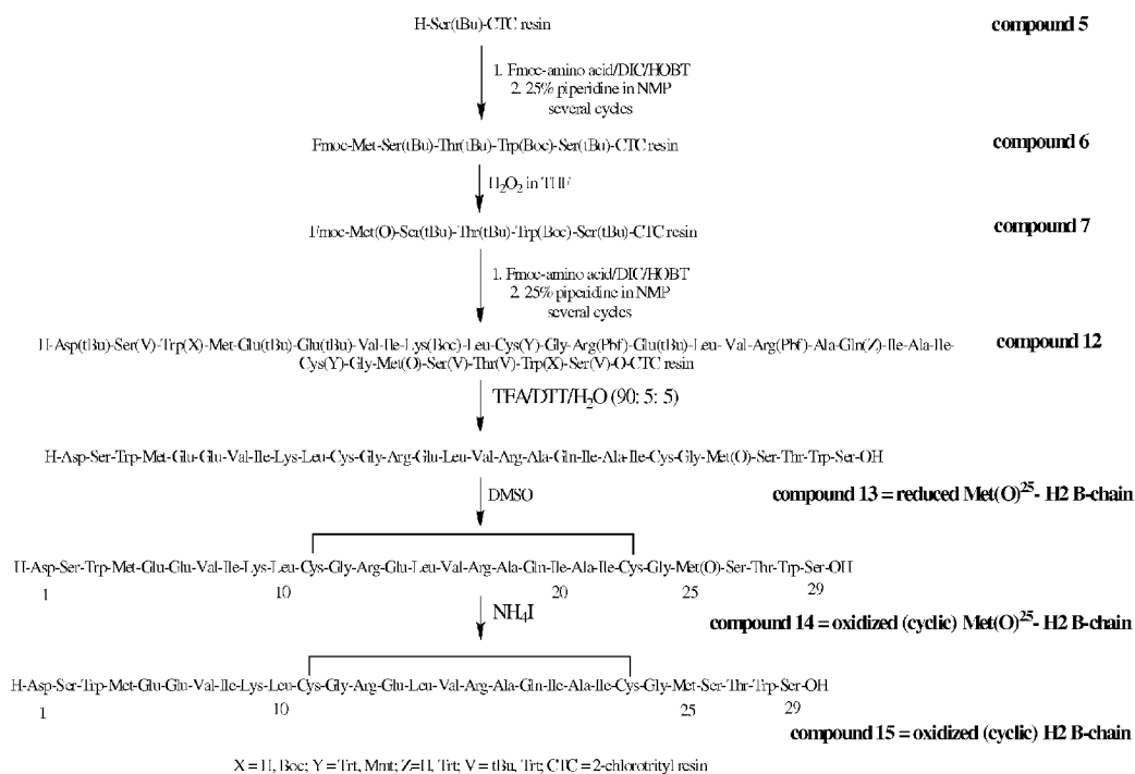
Figure 6. DMSO oxidation; Synthesis of reduced (linear) Met(O) 25 -human Relaxin 2 B-chain [ compound 13 , Met(O) 25 -shRLX2B], of oxidized (cyclic) Met(O) 25 -human Relaxin 2 B-chain [ compound 14 , Met(O) 25 -shRLX2B] and of oxidized (cyclic) human Relaxin 2 B-chain [ compound 15 , shRLX2B]
