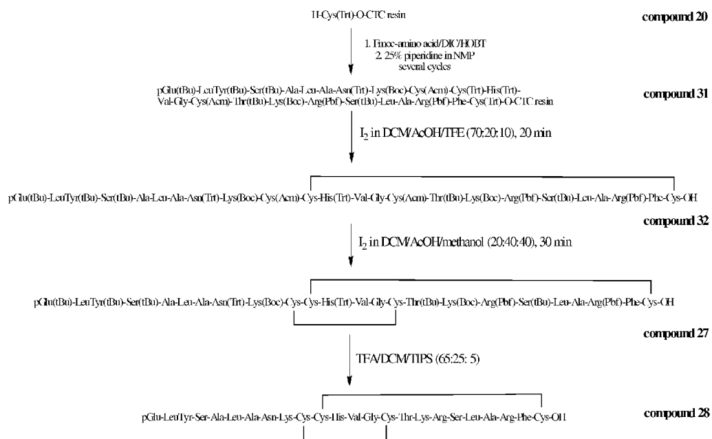
Figure 12. Synthesis of bicyclic human relaxin 2 chain A [compound 19; bicyclic RLX2A] with the application of S-Acm and Trt protecting groups
