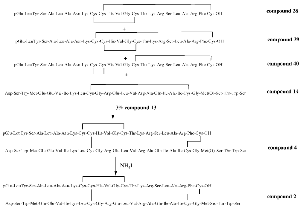
Figure 19. Synthesis of human relaxin 2 [RI.X2; compound 2 ] and of Met(O) 25 -human relaxin 2 [Met(O) 25 -RI.X2; compound 4 ] by chain combination of bicyclic RLX2A and cyclic Met(O) 25 -RLX2B)
