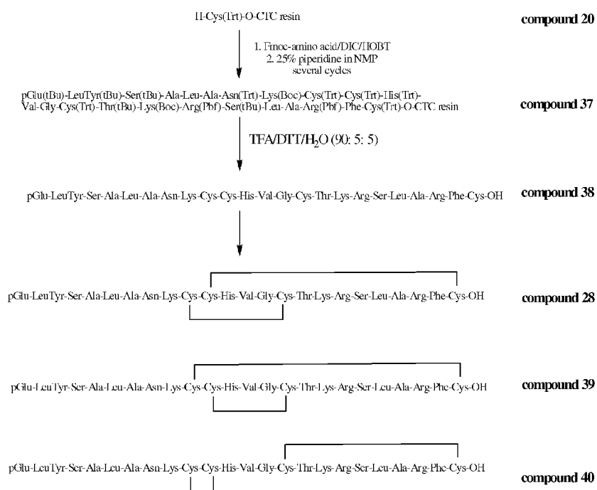
Figure 14. Synthesis of a mixture of bicyclic synthetic human relaxin 2 chains A [ compounds 28, 39-40 ; bicyclic RLX2A] by the DMSO oxidation of the linear chain
